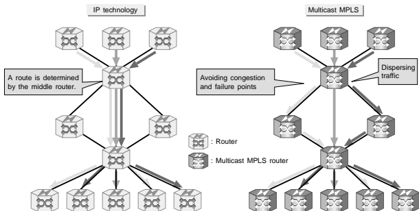
Fig. 2. Multicast traffic engineering functions.
